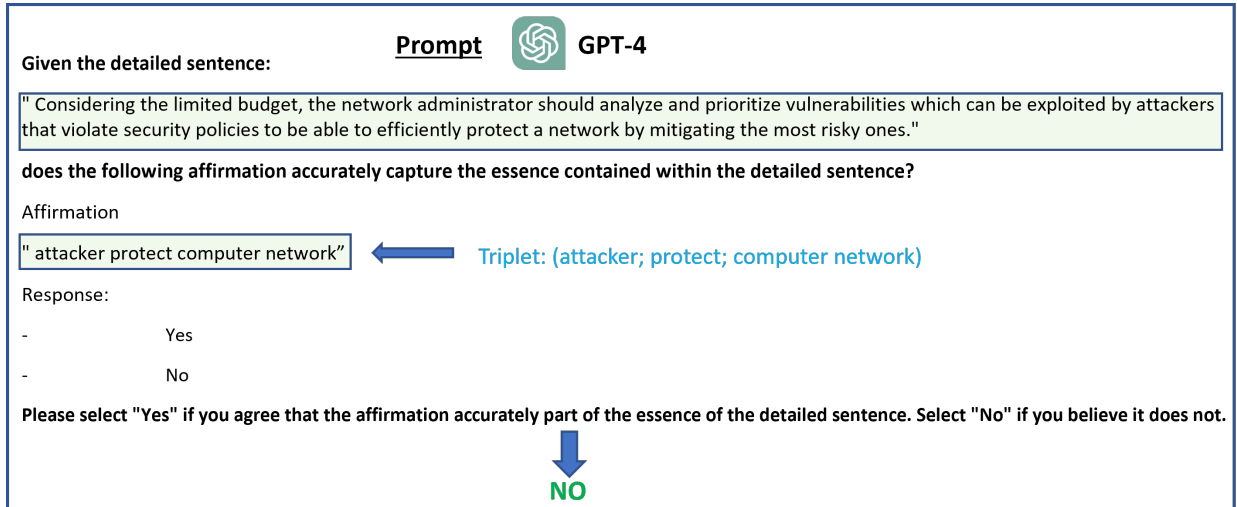
Fig. 3. Triplets Validation prompt
