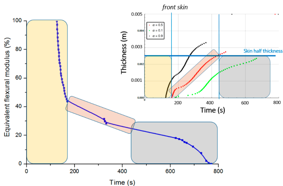
Figure 15. Apparent equivalent flexural modulus (contribution of only the front skin). Numerical predictions, considering a degradation rate gradient (see text for more details) as a function of time for an E-glass/vinyl ester/balsa sandwich composite material at a heat flux of 50 kW/m 2 . Inserted figure shows the prediction of the combustion advancing front in the front skin for three degradation levels \alpha(x, t) .
