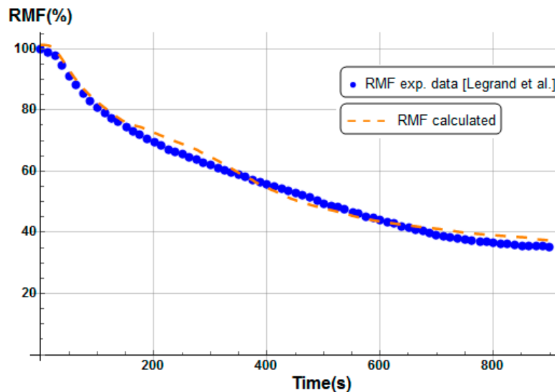
Figure 6. Remaining mass fraction (RMF) profile. Comparison between numerical prediction (this work) as a function of time and the experimental data from Legrand et al. [29] for an E-glass/polyester/balsa sandwich composite at a heat flux of 50 \text{ kW/m}^2 .
