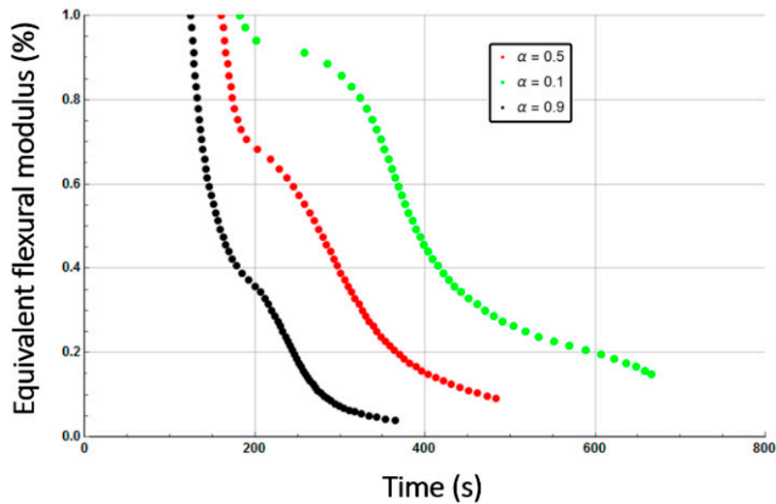
Figure 14. Apparent equivalent flexural modulus (contribution of only the front skin). Numerical predictions as a function of time for an E-glass/vinyl ester/balsa sandwich composite material at a heat flux of 50 kW/m 2 .
