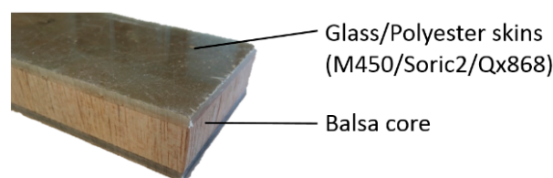
Figure 4. The E-glass/polyester/balsa sandwich composite specimen.
