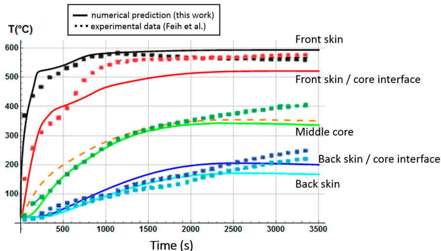
Figure 9. Temperature profiles. Comparison between our numerical prediction as a function of time (straight lines; average numerical temperature in orange dashed line) and the experimental data (dot points) from Feih et al. [34] for an E-glass/vinyl ester/balsa sandwich composite at a heat flux of 50 \text{ kW/m}^2 .
