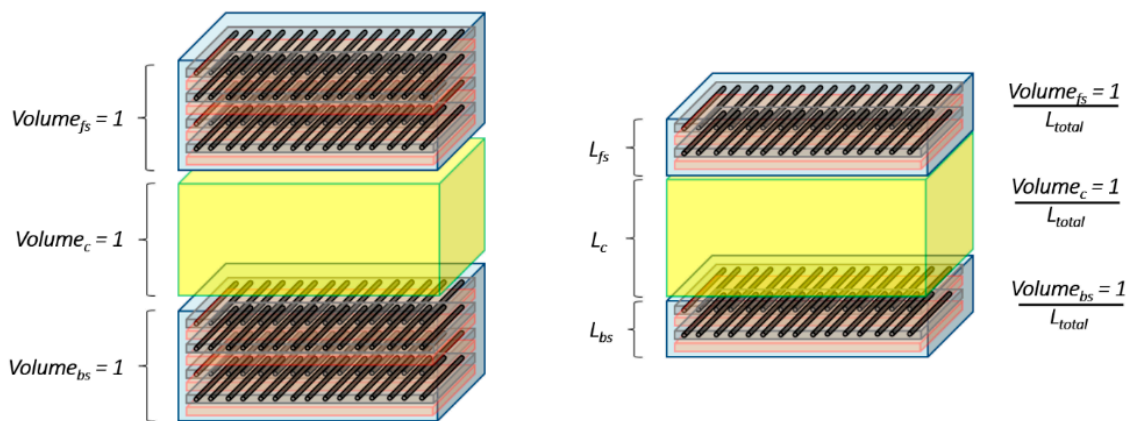
Figure 2. Scheme of the conversion of unit control volumes to real volumes in order to calculate the global mass of a composite sandwich material.
