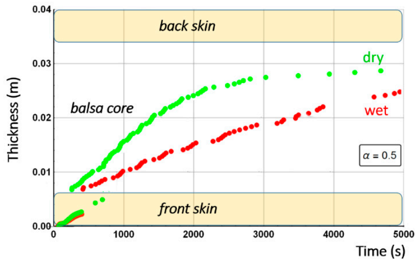
Figure 25. Prediction of the combustion advancing front for a moisturized E-glass/vinyl ester/balsa sandwich composite material (wet, red curve) at a heat flux of 50 \text{ kW/m}^2 , with a 20% water content in relation to the porosity volume fraction of the balsa core using the hygro-thermal model. Prediction comparison of the combustion advancing front for the same dry material (green curve).
