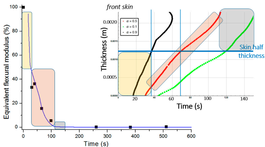
Figure 12. Apparent equivalent flexural modulus (contribution of only the front skin). Numerical predictions, considering a degradation rate gradient (see text for more details) as a function of time for an E-glass/polyester/balsa sandwich composite material at a heat flux of 50 kW/m 2 . Numerical predictions are superposed with the experimental data (■) measured by Legrand et al. [29]. Inserted figure shows the prediction of the combustion advancing front in the front skin for three degradation levels \alpha(x, t) .
