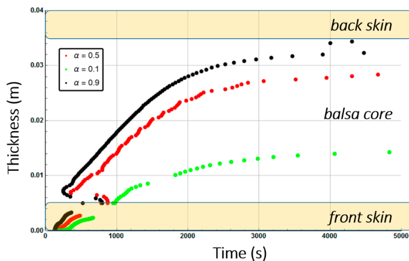
Figure 13. Numerical prediction of the combustion advancing front for an E glass/vinyl ester/balsa sandwich composite material at a heat flux of 50 \text{ kW/m}^2 : three degradation levels \alpha(x, t) are represented.
