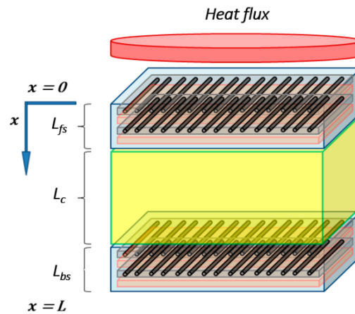
Figure 1. Scheme of thermal model for sandwich composite materials exposed to a constant unidirectional heat flux (balsa core in yellow; polymeric resin in orange; glass fibers in black).
