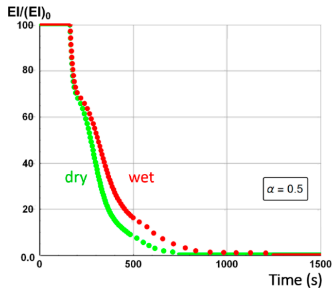
Figure 26. Post-combustion time dependence of the normalized flexural modulus. Comparison of numerical predictions as a function of combustion time between pure thermal (dry sample, green curve) and hygro-thermal (wet sample, red curve; 20% water content in relation to the porosity volume fraction of the balsa core) models for an E-glass/vinyl ester/balsa sandwich composite at a heat flux of 50 \text{ kW/m}^2 and for a degradation level of 50%.
