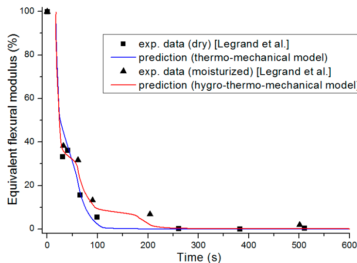
Figure 22. Post-combustion time dependence of the equivalent flexural modulus, considering a degradation rate gradient. Comparison of numerical prediction between thermal and hygro-thermal models for an E-glass/polyester/balsa sandwich composite at a heat flux of 50 \text{ kW/m}^2 . The experimental data for both specimens (dry and moisturized) [29] are also shown.
