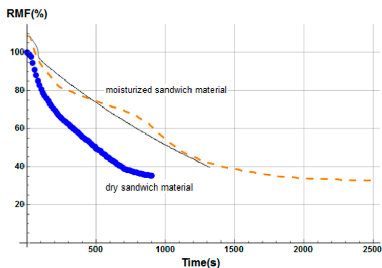
Figure 17. Remaining mass fraction (RMF) profile. Comparison of the numerical predictions as a function of time between thermal (blue dot line) and hygro-thermal (orange dashed line) models. Experimental data from Legrand et al. [29] are added (black line) for the moisturized sandwich material. Compound: E-glass/polyester/balsa sandwich composite at a heat flux of 50 kW/m 2 .
