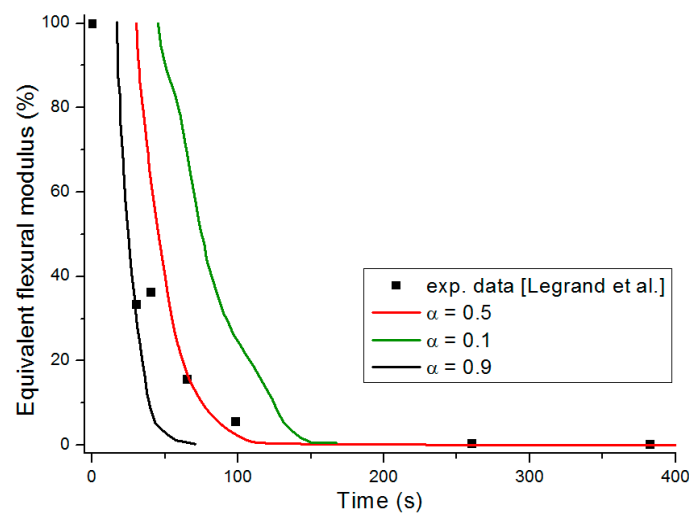
Figure 11. Apparent equivalent flexural modulus (contribution of only the front skin). Numerical simulation predictions as a function of time for an E-glass/polyester/balsa sandwich composite material at a heat flux of 50 kW/m 2 . Numerical predictions are superposed with the experimental data (■) measured by Legrand et al. [29].
