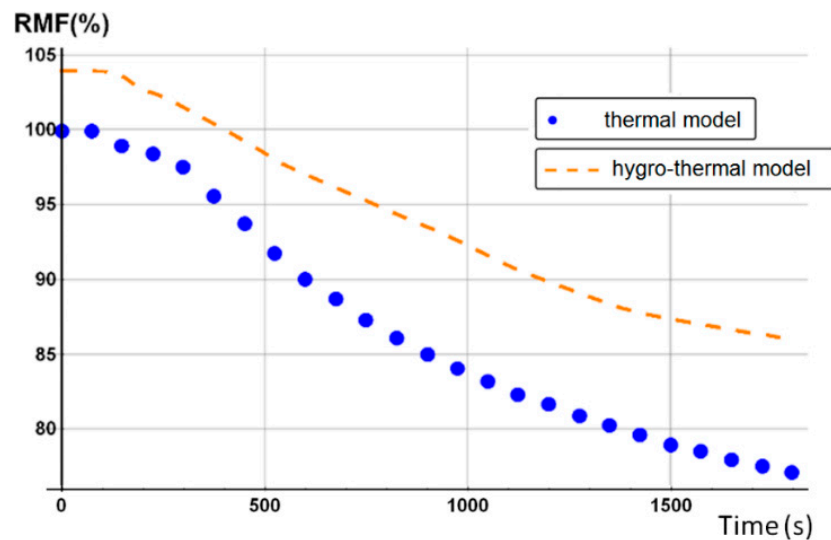
Figure 23. Remaining mass fraction (RMF) profile. Comparison of the numerical predictions as a function of time between thermal (blue dot line) and hygro-thermal (orange dashed line) models for an E-glass/vinyl ester/balsa sandwich composite at a heat flux of 50 \text{ kW/m}^2 .
