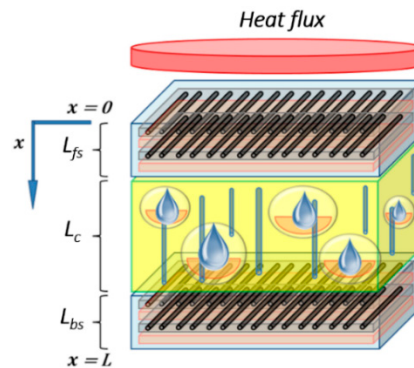
Figure 16. Scheme of the hygro-thermal model for sandwich composite material exposed to a constant unidirectional heat flux. The model considers the presence of (i) porosities and moisture absorption inside the skins, and of (ii) porosities, resin diffusion and moisture absorption inside the balsa core.
