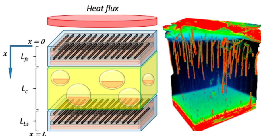
Figure 5. Scheme of thermal model for sandwich composites exposed to a constant unidirectional heat flux considering resin diffusion inside the balsa: each sandwich core volume element is constituted by balsa material + porosity (air) + resin (skin polymeric matrix). \mu -tomographic 3D-image reconstruction obtained on a for E-glass/polyester/balsa sandwich composite sample (XRADIA instrument, 15 s exposure time, pixel size 12.6 \mu\text{m} , 721 images).
