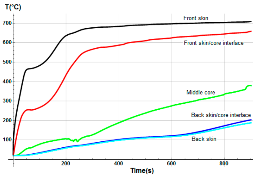
Figure 18. Temperature profile for an E-glass/polyester/balsa sandwich composite with a 30% water content in relation to the porosity volume fraction of the balsa core, at a heat flux of 50 kW/m 2 .
