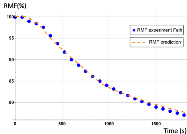
Figure 8. Remaining mass fraction (RMF) profile. Comparison between numerical prediction (this work) as a function of time and the experimental data from Feih et al. [34] for an E-glass/vinyl ester/balsa sandwich composite at a heat flux of 50 \text{ kW/m}^2 .
