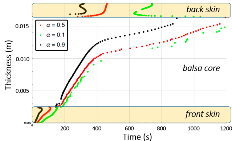
Figure 10. Numerical simulation prediction of the combustion advancing front for an E-glass/polyester/balsa sandwich composite material at a heat flux of 50 \text{ kW/m}^2 : three degradation levels \alpha(x, t) are represented.
