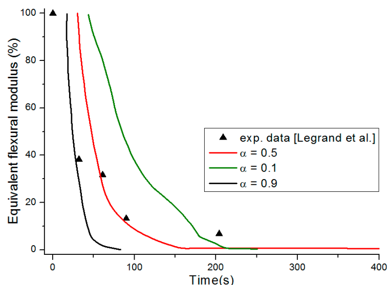
Figure 20. Apparent equivalent flexural modulus (contribution of only the front skin). Numerical simulation predictions as a function of time for an E-glass/polyester/balsa moisturized sandwich composite material at a heat flux of 50 \text{ kW/m}^2 . Numerical predictions are superposed with the experimental data ( \blacktriangle ) measured by Legrand et al. [29].
