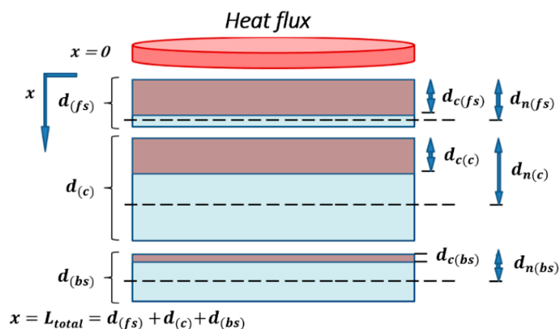
Figure 3. Scheme of the idealized two-layer approach for each constituent in order to study the post-combustion mechanical properties of a sandwich composite material. The decomposed constituent material (char material, in brown) and virgin material (in blue) evolve as a function of time and temperature through the specimen thickness direction x (combustion advancing front).
