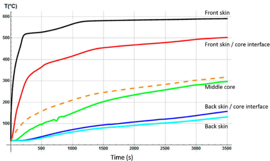
Figure 24. Temperature profiles prediction as a function of time (straight lines; average numerical temperature in orange dashed line) for an E-glass/vinyl ester/balsa sandwich composite, with a 20% water content in relation to the porosity volume fraction of the balsa core, at a heat flux of 50 kW/m 2 .
