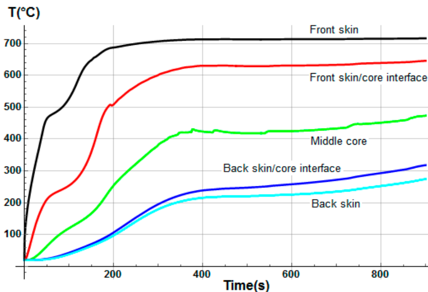
Figure 7. Temperature profile for an E glass/polyester/balsa sandwich composite at a heat flux of 50 \text{ kW/m}^2 .
