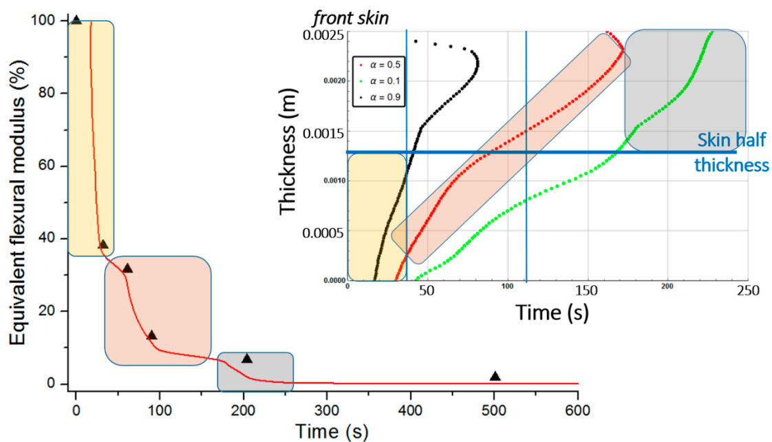
Figure 21. Apparent equivalent flexural modulus (contribution of only the front skin). Numerical predictions, considering a degradation rate gradient (see text for more details) as a function of time for a moisturized E-glass/polyester/balsa sandwich composite material at a heat flux of 50 \text{ kW/m}^2 . Numerical predictions are superposed with the experimental data ( \blacktriangle ) measured by Legrand et al. [29]. Insert shows prediction of the combustion advancing front in the front skin for three degradation levels \alpha(x, t) .
