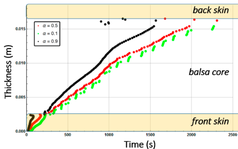
Figure 19. Numerical simulation prediction of the combustion advancing front for a moisturized E-glass/polyester/balsa sandwich composite material at a heat flux of 50 \text{ kW/m}^2 , using the hygro-thermal model.
