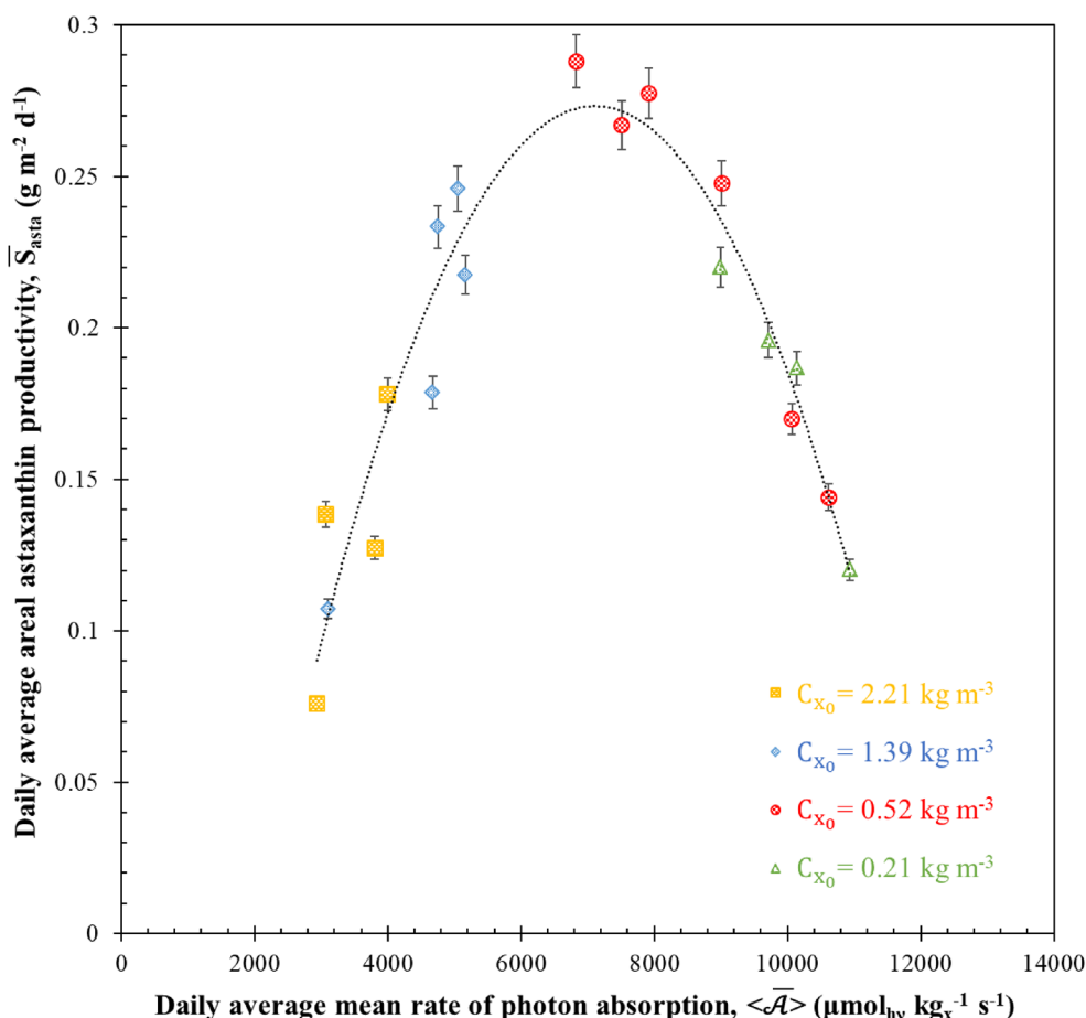
Fig. 7 Evolution of daily average areal astaxanthin productivity \bar{S}_{asta} of H. pluvialis during sudden nitrogen starvation of batch cultures exposed to PFD of 250 \text{ } \mu\text{mol}_{\text{hv}} \text{ m}^{-2} \text{ s}^{-1} with initial biomass concentrations C_{x_0} equals to 0.21, 0.52, 1.39 and 2.21 \text{ kg m}^{-3} as a function of daily average mean rate of photon absorption \langle \bar{A} \rangle . Data shown as mean \pm SD, n=3
