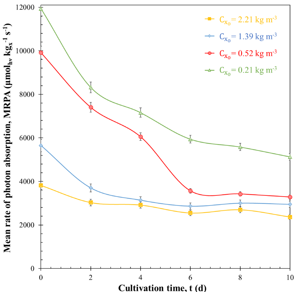
Fig. 6 The mean rate of photon absorption MRPA of H. pluvialis during sudden nitrogen starvation of batch cultures exposed to PFD of 250 \text{ } \mu\text{mol}_{hv} \text{ m}^{-2} \text{ s}^{-1} with initial biomass concentrations C_{x_0} equals to 0.21, 0.52, 1.39 and 2.21 \text{ kg m}^{-3} as a function of cultivation time t . Data shown as mean \pm SD, n = 3
