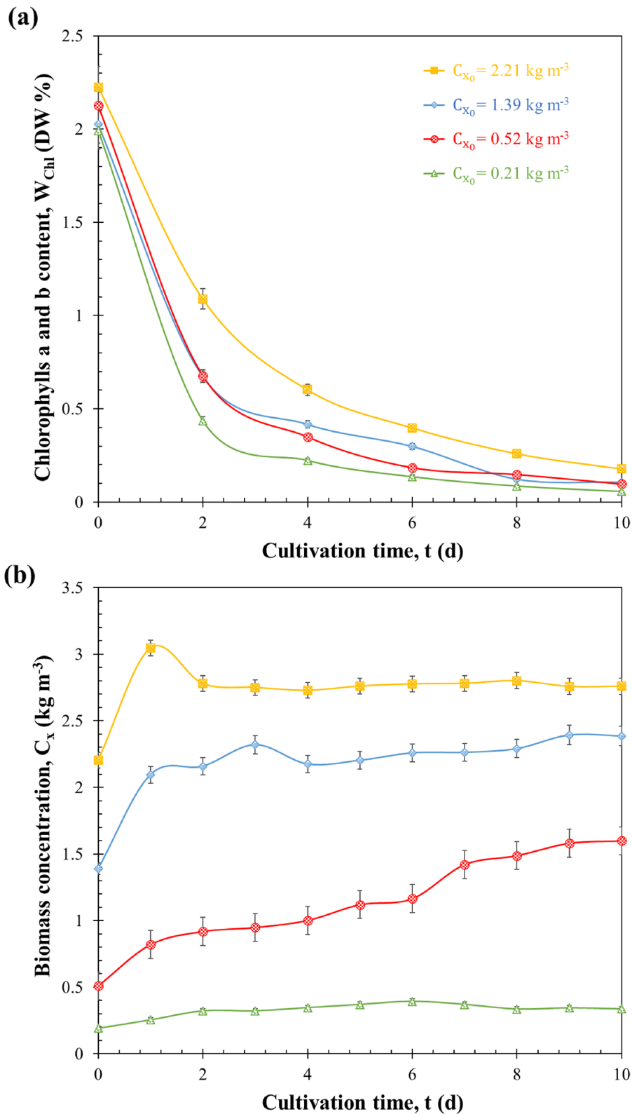
Fig. 1 Chlorophyll content W_{chl} (a) and biomass concentration C_x (b) of H. pluvialis during sudden nitrogen starvation of batch cultures exposed to PFD of 250\ \mu mol_{hv}\ m^{-2}\ s^{-1} with initial biomass concentrations C_{x_0} equals to 0.21, 0.52, 1.39 and 2.21\ kg\ m^{-3} as a function of cultivation time t . Data shown as mean \pm SD, n=3
