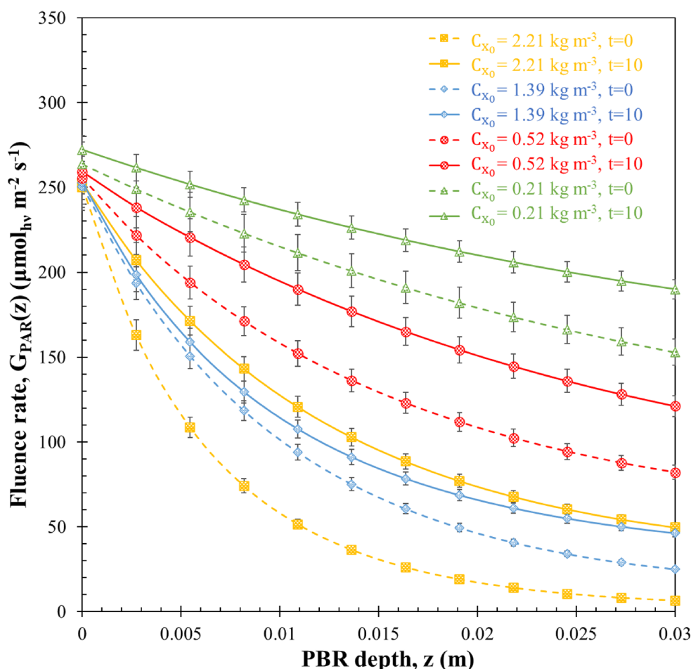
Fig. 5 The PAR-averaged fluence rate G(z) of H. pluvialis at the start ( t=0 ) and the end ( t=10 ) of sudden nitrogen starvation of batch cultures exposed to PFD of 250 \mu\text{mol}_{hv} \text{m}^{-2} \text{s}^{-1} with initial biomass concentrations C_{x_0} equals to 0.21, 0.52, 1.39 and 2.21 \text{kg m}^{-3} as a function of PBR depth z . Data shown as mean \pm SD, n=3
