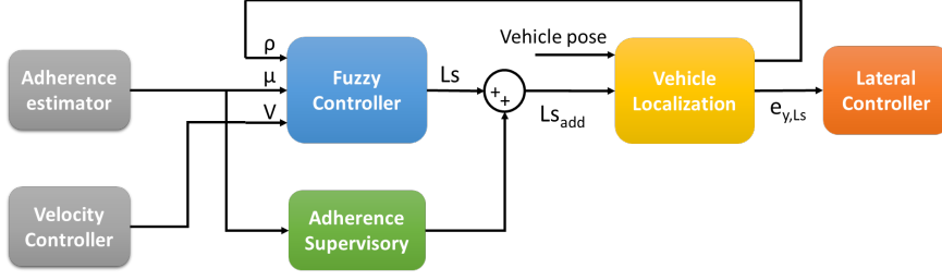
Figure 12.: Fuzzy control scheme
