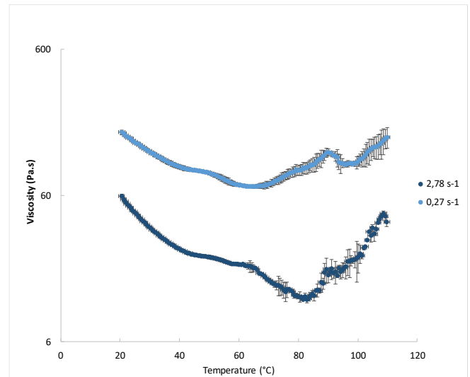
Figure 4. Viscosity of the cake batter vs temperatures for two shear rates
