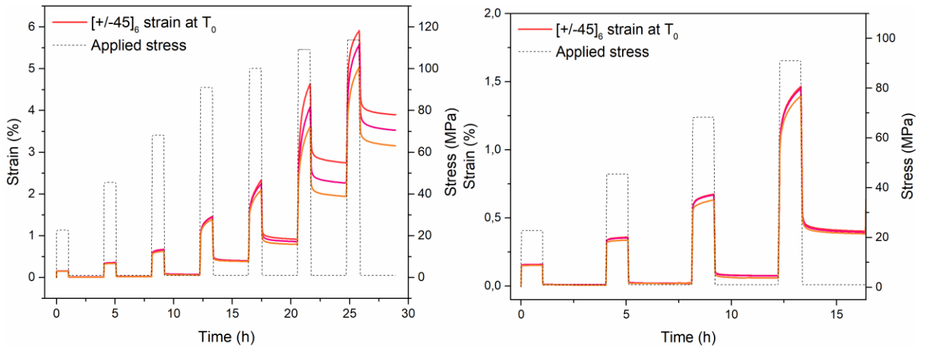
Figure 4: Creep-recovery tests at T_0 for the 7 step creep-recovery sequence (left) and focus on the first four steps (right).
