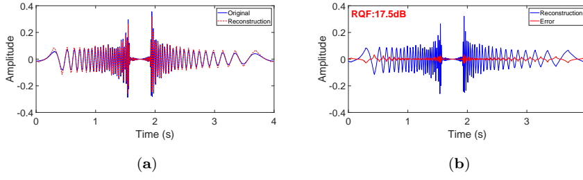
Fig. 8: (a) The original signal and the reconstructed signal, (b) The reconstructed signal and the reconstructed error.
