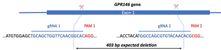
Figure 1. Guide RNAs design for the deletion of GPR146
