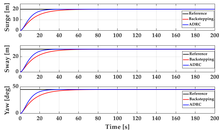
Figure 12. The position of surge, sway and yaw under ideal sea condition.
