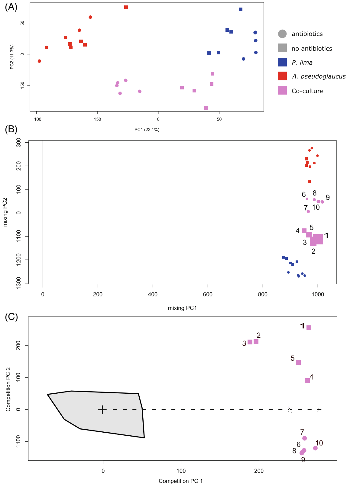
FIGURE 3 Unsupervised data analysis ( n = 5 ) of LC-HRMS data showing differences between Prochlorococcus lima , Aspergillus pseudoglaucus and their co-culture samples, in absence or presence of antibiotics. (A) Principal component analysis (log transformed data, pareto scaling); (B) Mixing model using Projected Orthogonalised Encounter Monitoring (POChEMon) data analysis (Jansen et al., 2015). In the mixing model, the size of the co-culture samples reflects the amount of their unexplained variance within the mixing model (the larger the point, the higher the unexplained variance); (C) Competition model using Projected Orthogonalised Encounter Monitoring (POChEMon) data analysis. The grey zone corresponds to the projected co-culture domain within the competition model.
