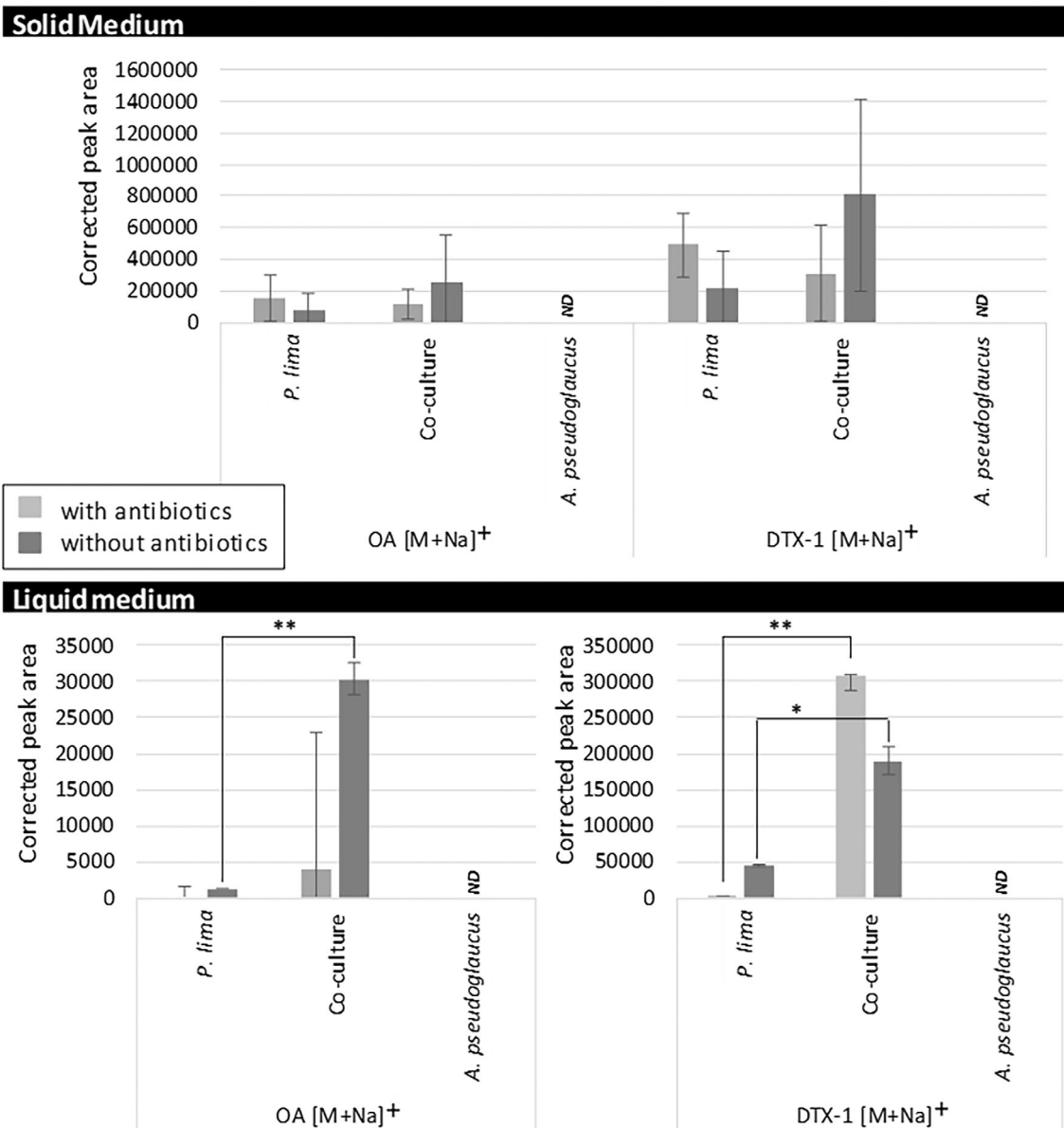
FIGURE 4 Okadaic acid (OA) [M + Na] + ( m/z = 827.463 ) and dinophysistoxin 1 (DTX-1) [M + Na] + ( m/z = 841.473 ) corrected peak area (peak area corrected by amount of extract) detected within LC-HRMS data in positive ionization mode according to the type of samples where it was detected. (ND: not detected; variation significance based on student test: * p -value \leq 0.05 , ** p -value \leq 0.01 )
