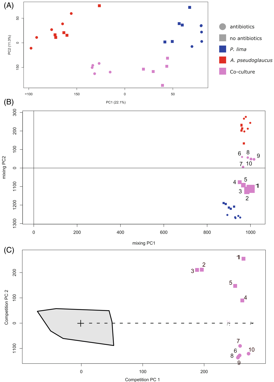
FIGURE 3 Unsupervised data analysis ( n = 5 ) of LC-HRMS data showing differences between Proocentrum lima , Aspergillus pseudoglaucus and their co-culture samples, in absence or presence of antibiotics. (A) Principal component analysis (log transformed data, pareto scaling); (B) Mixing model using Projected Orthogonalised Encounter Monitoring (POChEMon) data analysis (Jansen et al., 2015). In the mixing model, the size of the co-culture samples reflects the amount of their unexplained variance within the mixing model (the larger the point, the higher the unexplained variance); (C) Competition model using Projected Orthogonalised Encounter Monitoring (POChEMon) data analysis. The grey zone corresponds to the projected co-culture domain within the competition model.
