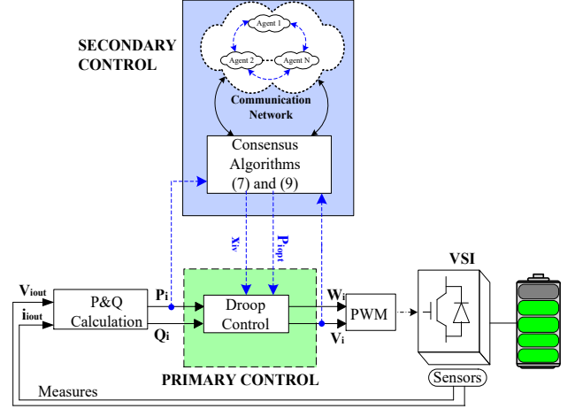
Fig. 3. DG control scheme
