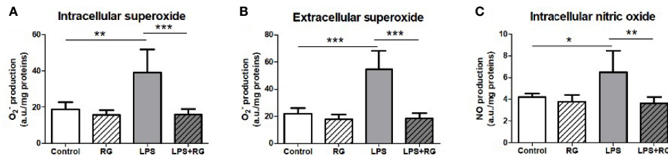
FIGURE 2 | LPS treatment of FaO rat hepatoma cells resulted in increased superoxide concentration, both intracellularly ( A ), and extracellularly ( B ), as well as increased intracellular nitric oxide concentration ( C ). Oxide increases were diminished by RG100204 treatment. The levels of O 2 - and NO were assayed by electron paramagnetic resonance of spin traps prepared from the FaO cells submitted to the different experimental conditions. Control, cells exposed to the vehicle (1% DMSO) alone; RG, 25 μM RG100204 in 1% DMSO; LPS, 1 μg LPS/mL in 1% DMSO; LPS+RG, 25 μM RG100204 plus 1 μg LPS/mL in 1% DMSO; a.u., arbitrary units. Data were analyzed by one-way ANOVA, with Bonferroni's post-hoc test. Data are expressed as mean ± SEM, n=5, *P < 0.05, **P < 0.01 and ***P < 0.001.
