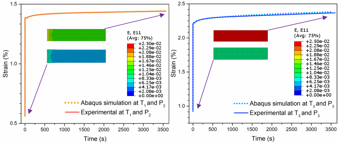
Fig 14: Hygro-viscoelastic simulations and experimental comparisons of longitudinal strain for two creep stages P_2 and P_3
