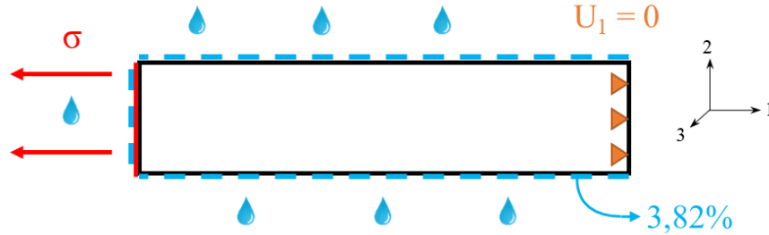
Fig 12: Scheme of the resin subjected to both water diffusion and applied stress
