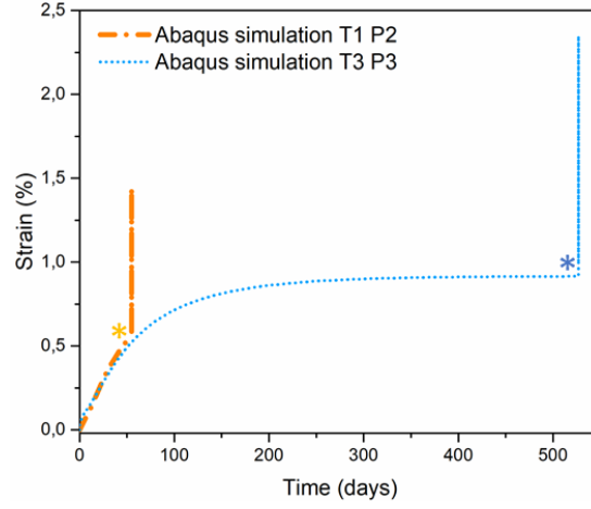
Fig 13: Evolution of the total longitudinal strain: hygro-viscoelastic simulations for time T_1 associated to load P_2 and time T_3 associated to load P_3
