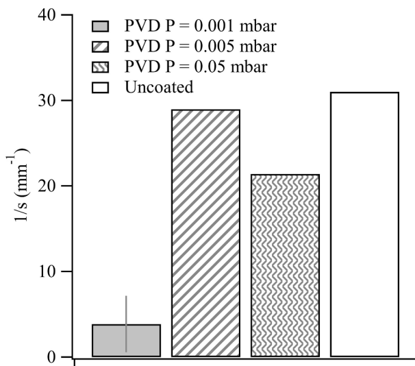
Fig. 3. 1/s parameter for coated and uncoated nickel multicrystal. 1/s of polycrystals = 0.
