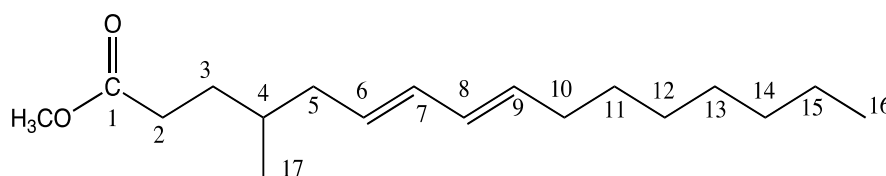
Scheme 1. Chemical structure of 4-Me-6E,8E-16:2 methyl ester.
