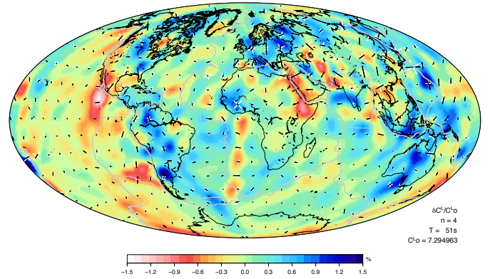
Figure A2. Phase velocity distributions of the different Love wave higher modes at the same period ( T = 51 s).
