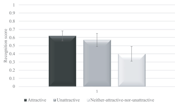
Fig. 2. Recognition scores for attractive faces, unattractive faces, and neither-attractive-nor-unattractive faces.
