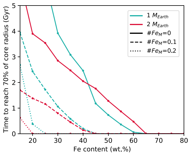
Figure 10. Time required for the solid inner core to reach 70% of the core radius as a function of bulk iron content, for planets with 1 and 2 M_{\text{Earth}} and different mantle iron numbers \#Fe_M . The core is made of pure iron. For planets with low iron contents (bulk and mantle) the inner core does not reach 70% of the core radius during 5 Gyr of evolution.
