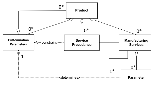
Fig.1. UML Product Manufacturing-Model
